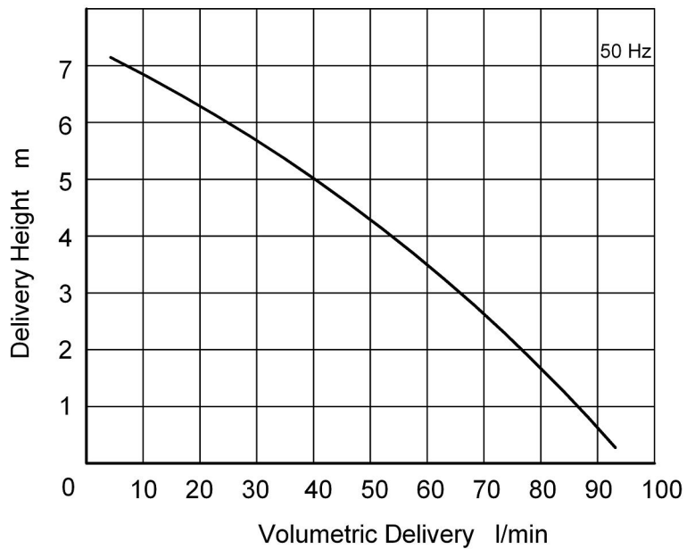
Performance Curve
